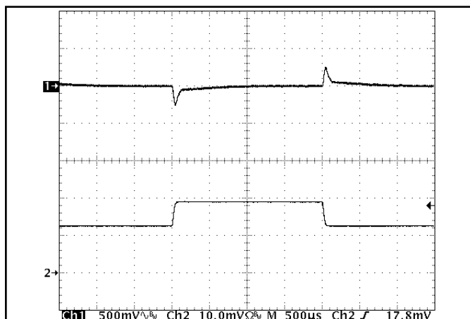
Figure 11: Output voltage response to step-change in load current (50%-75%-50%) of I_{out(max)} : dI/dt = 0.16A/\mu s . Load cap: 10μF, 100 mΩ ESR tantalum cap and 1μF ceramic cap. Ch 1: V_{out} (500mV/div), Ch 2: I_{out} (10A/div).
