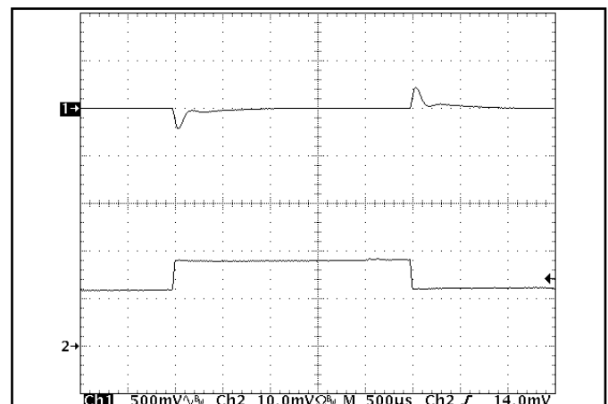
Figure 12: Output voltage response to step-change in load current (50%-75%-50%) of I_{out(max)} : dI/dt = 0.4A/\mu s . Load cap: 470μF, 30 mΩ ESR tantalum cap and 1μF ceramic cap. Ch 1: V_{out} (500mV/div), Ch 2: I_{out} (10A/div).
