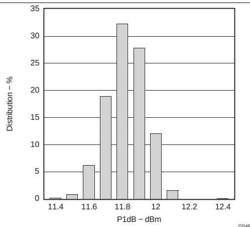
Figure 43. P1dB at 1800 MHz Distribution
