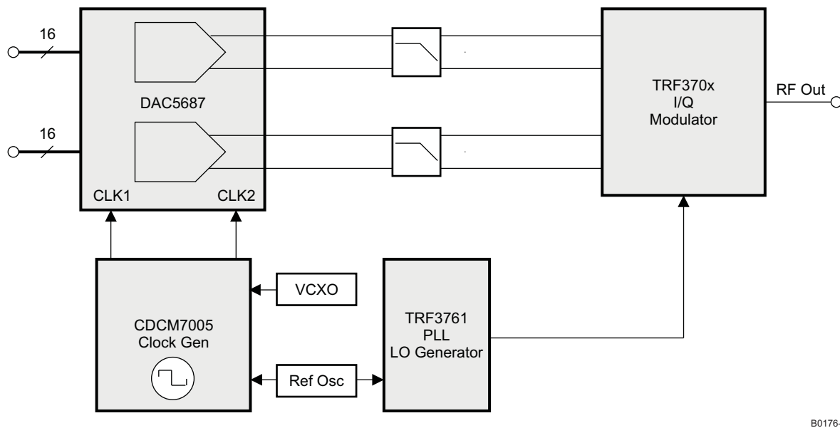
Figure 45. Typical Transmit Setup Block Diagram
