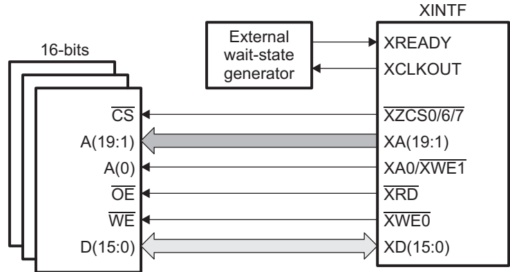
Figure 4-21. Typical 16-bit Data Bus XINTF Connections
