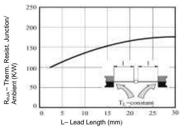
Figure2. Thermal Resistance vs. Lead Length
