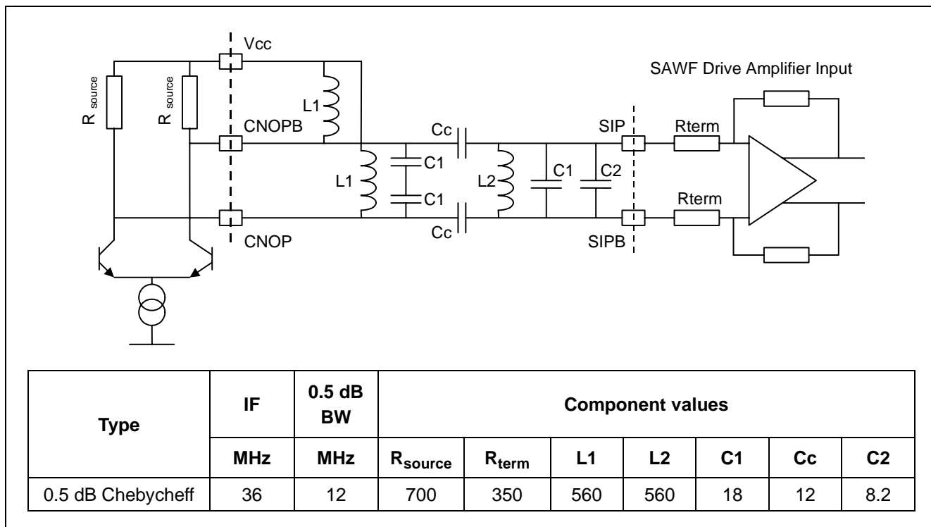
Figure 9 - Interstage Filter
