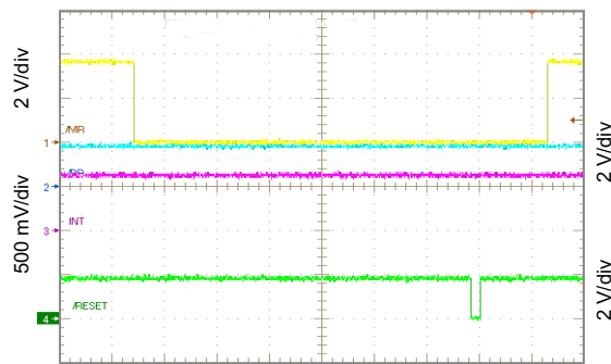
图 101. \overline{\text{RESET}} Timing
