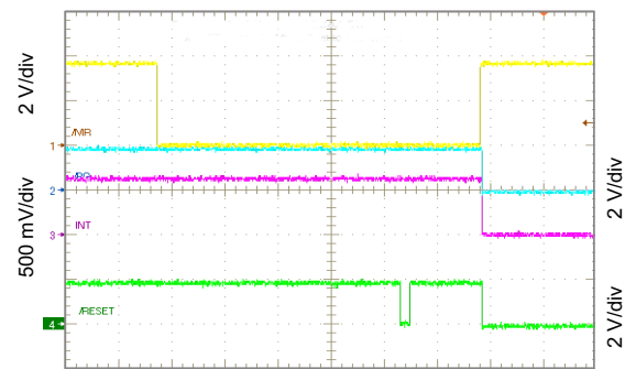
图 102. \overline{\text{RESET}} Timing
