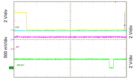
图 102. \overline{\text{RESET}} Timing
