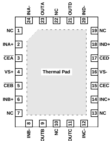
EL5493A (24-PIN LPP) TOP VIEW
