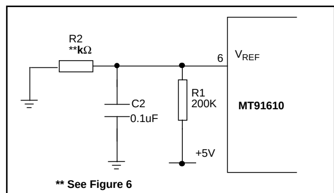
Figure 3 - Loop Setting
