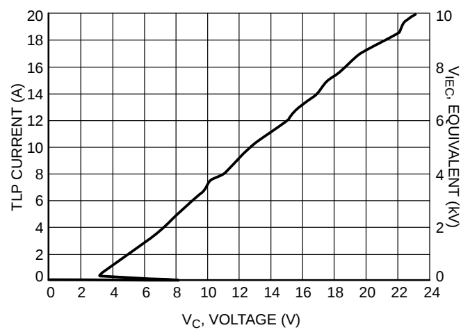
Figure 2. Positive TLP I-V Curve
