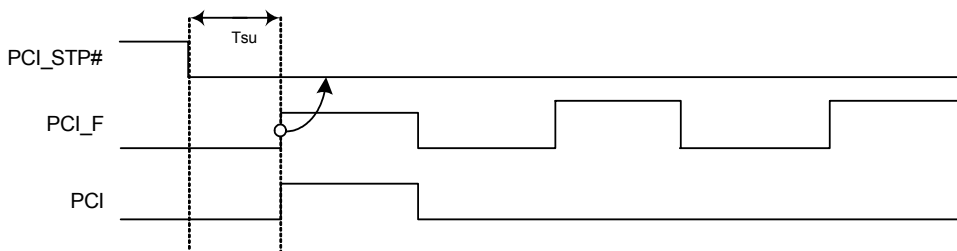
Figure 7. PCI_STP# Assertion Waveform
