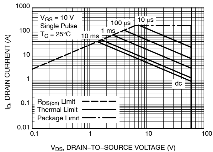
Figure 11. Maximum Rated Forward Biased Safe Operating Area
