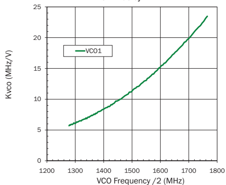
VC01 Frequency versus Kvco LO Divide by 2
