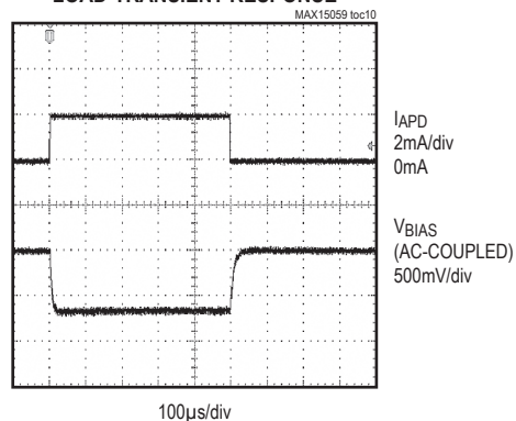
LOAD-TRANSIENT RESPONSE
