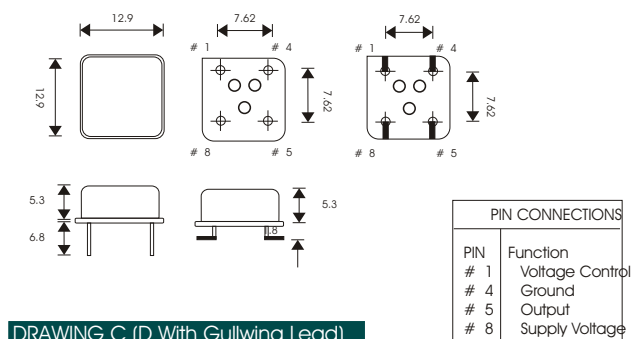
DRAWING C (D With Gullwing Lead)
