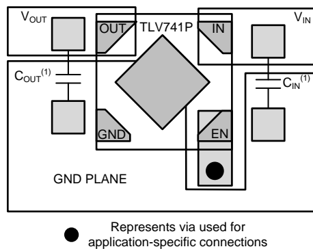
Figure 34. Layout Example: DBV Package
