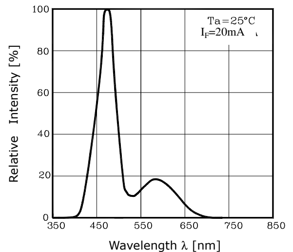
Fig. 4 Spectrum Distribution
