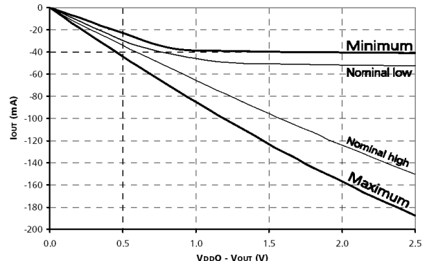
Figure 10: Pull-Up Characteristics
