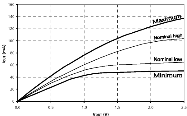
Figure 9: Pull-Down Characteristics
