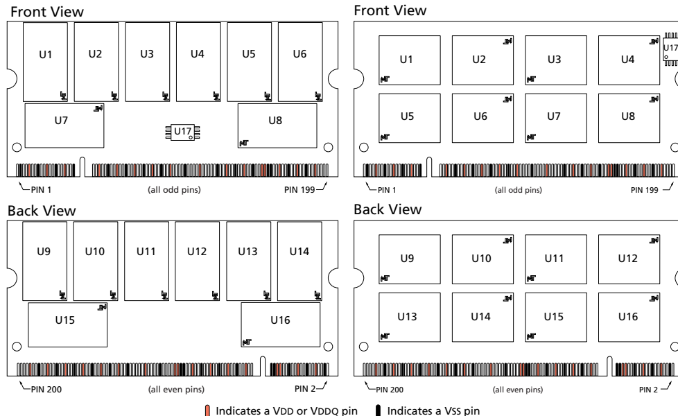
Figure 2: Module Layout
