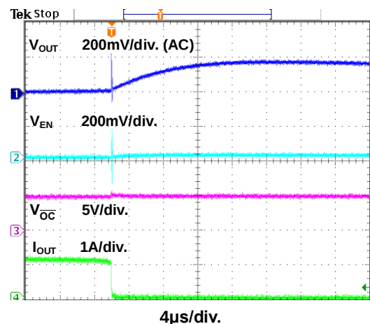
Figure 14. Output Load Insert Hot Plug-Off with 3.8\Omega (1.3A)
