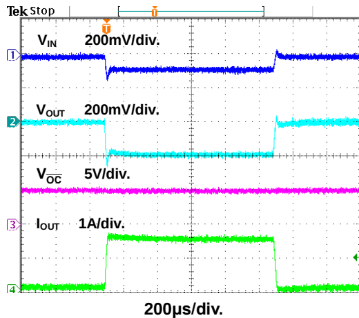
Figure 11. Load transient
