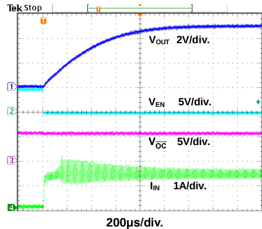
Figure 6. EN Start-Up
