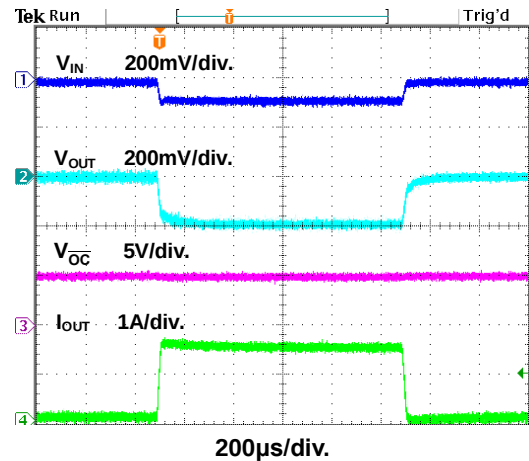
Figure 12. Load transient
