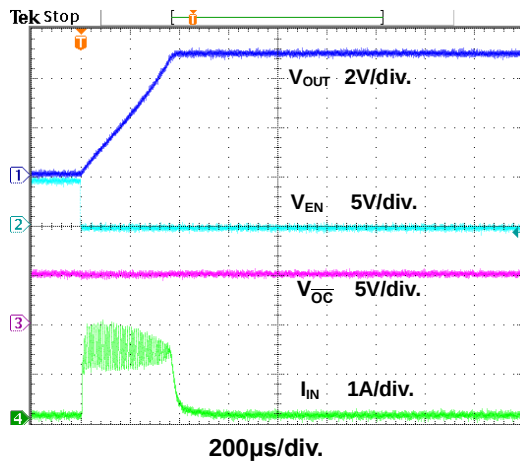
Figure 5. EN Start-Up
