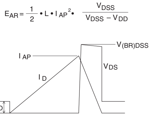
Avalanche Waveform
