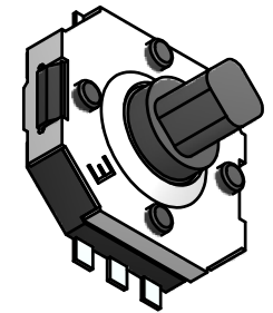
ISOMETRIC
