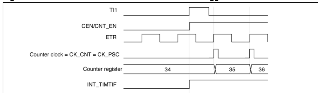
Figure 39. Control circuit in external clock mode 2 + trigger mode
