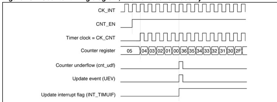
Figure 16. Counter timing diagram, internal clock divided by 1
