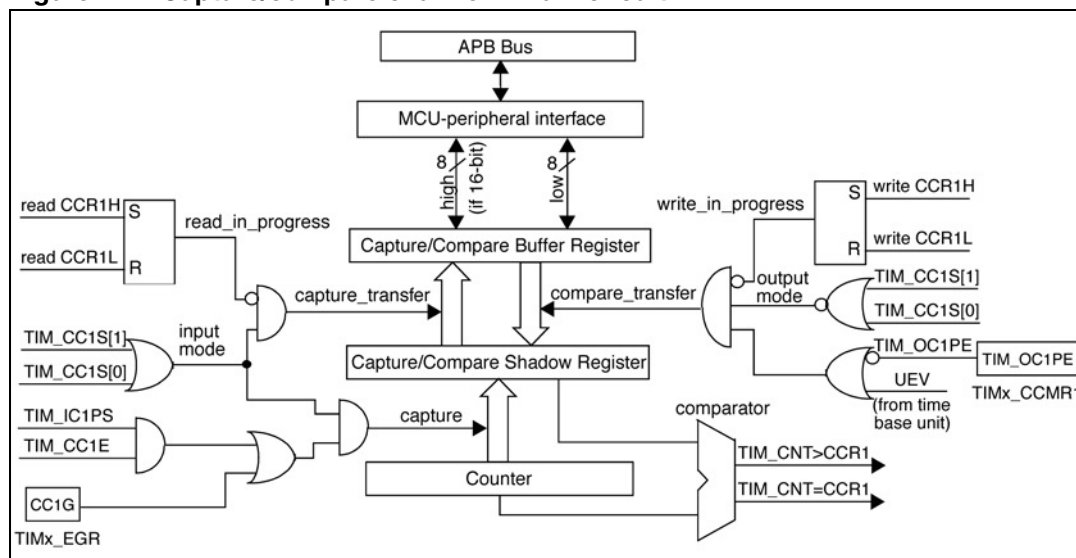
Figure 27. Capture/compare channel 1 main circuit
