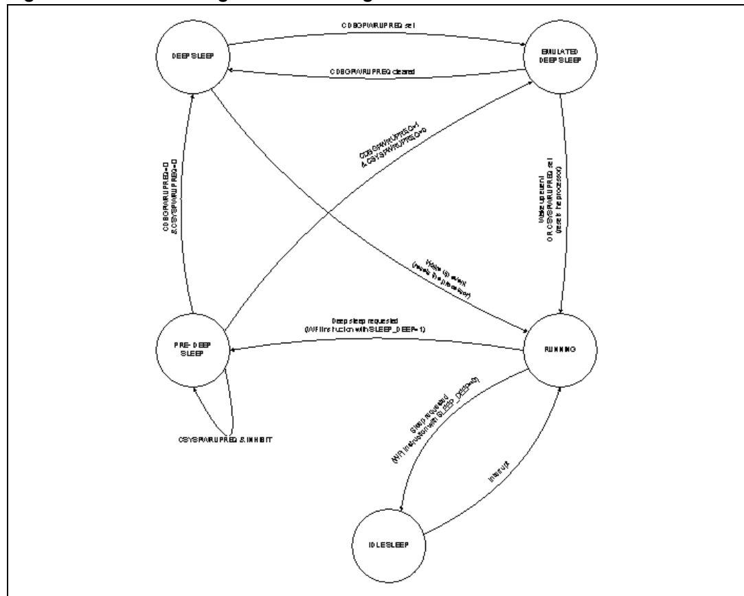
Figure 7. Power management state diagram
