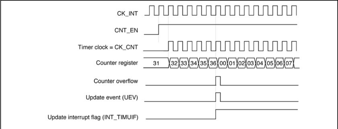
Figure 12. Counter timing diagram, internal clock divided by 1
