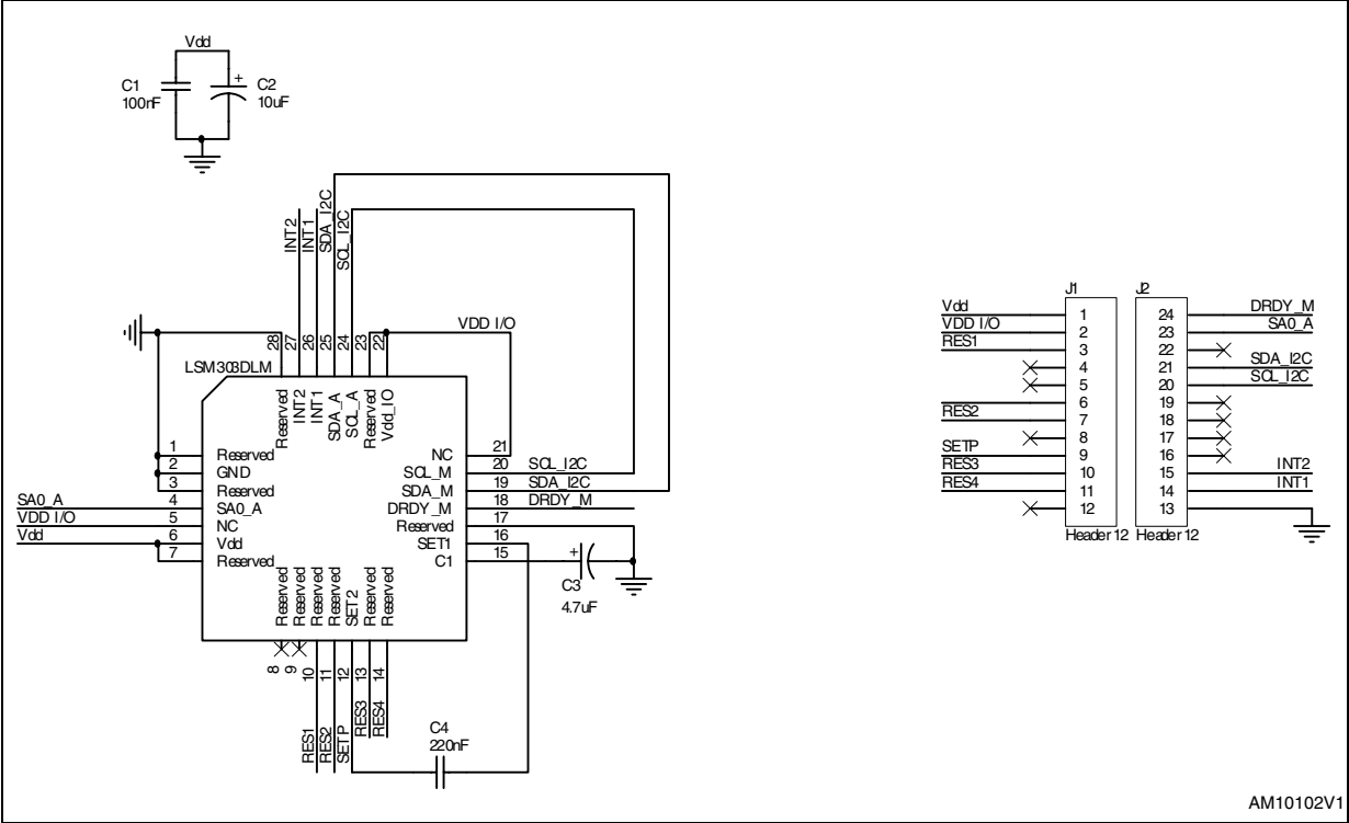
Figure 1. Schematic circuit
