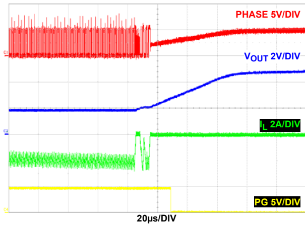
FIGURE 51. OVERVOLTAGE PROTECTION
