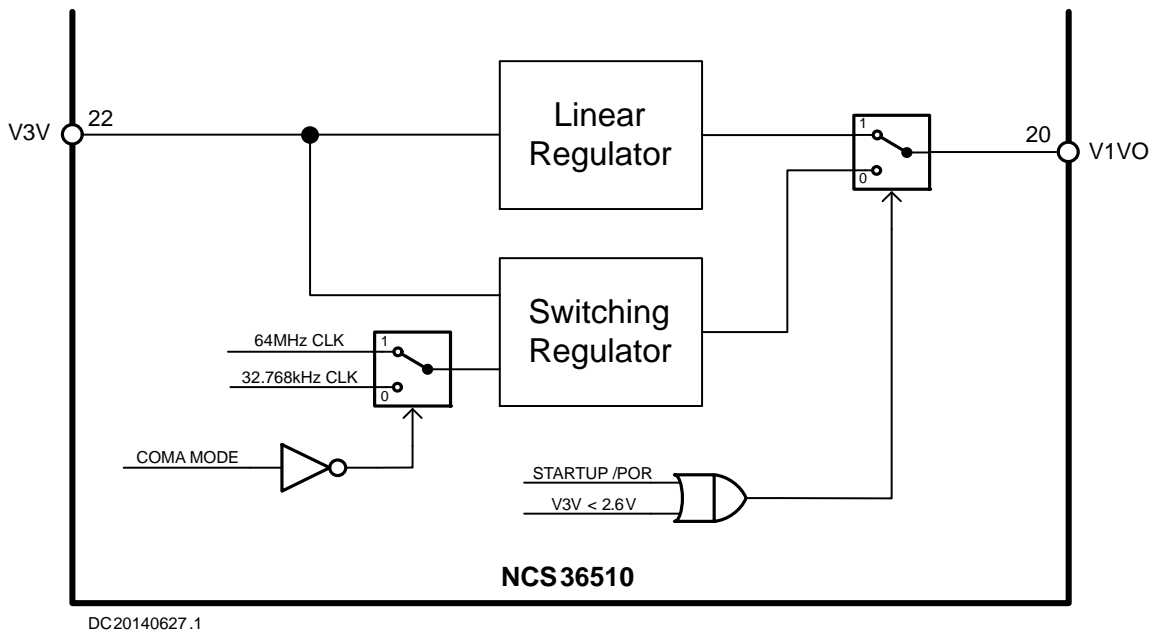
Figure 9. Pre-Regulator System
