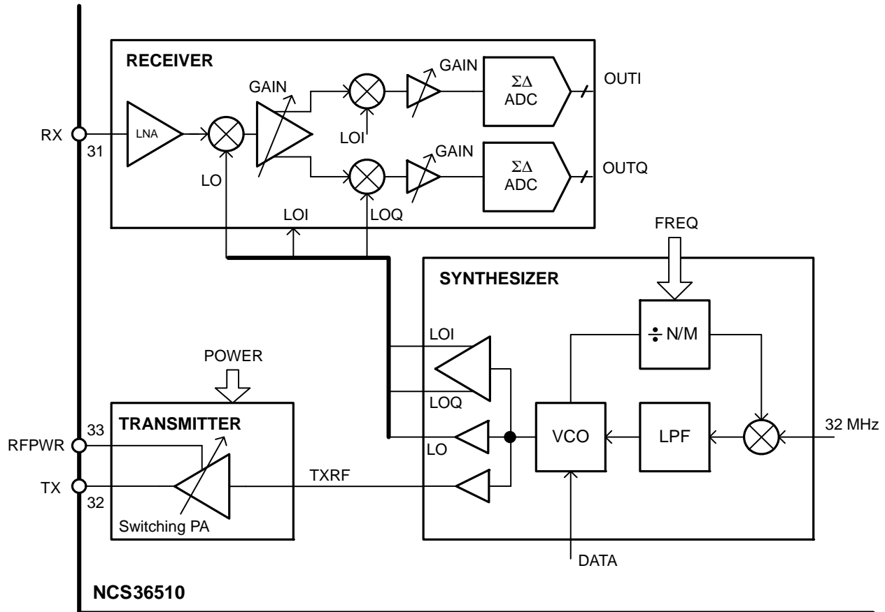
Figure 5. Radio Block Diagram
