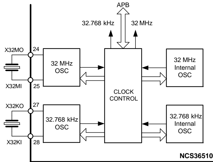
Figure 4. Clock System
