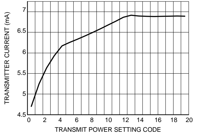
Figure 22. 1 V Mode Transmitter Current versus Power Setting
