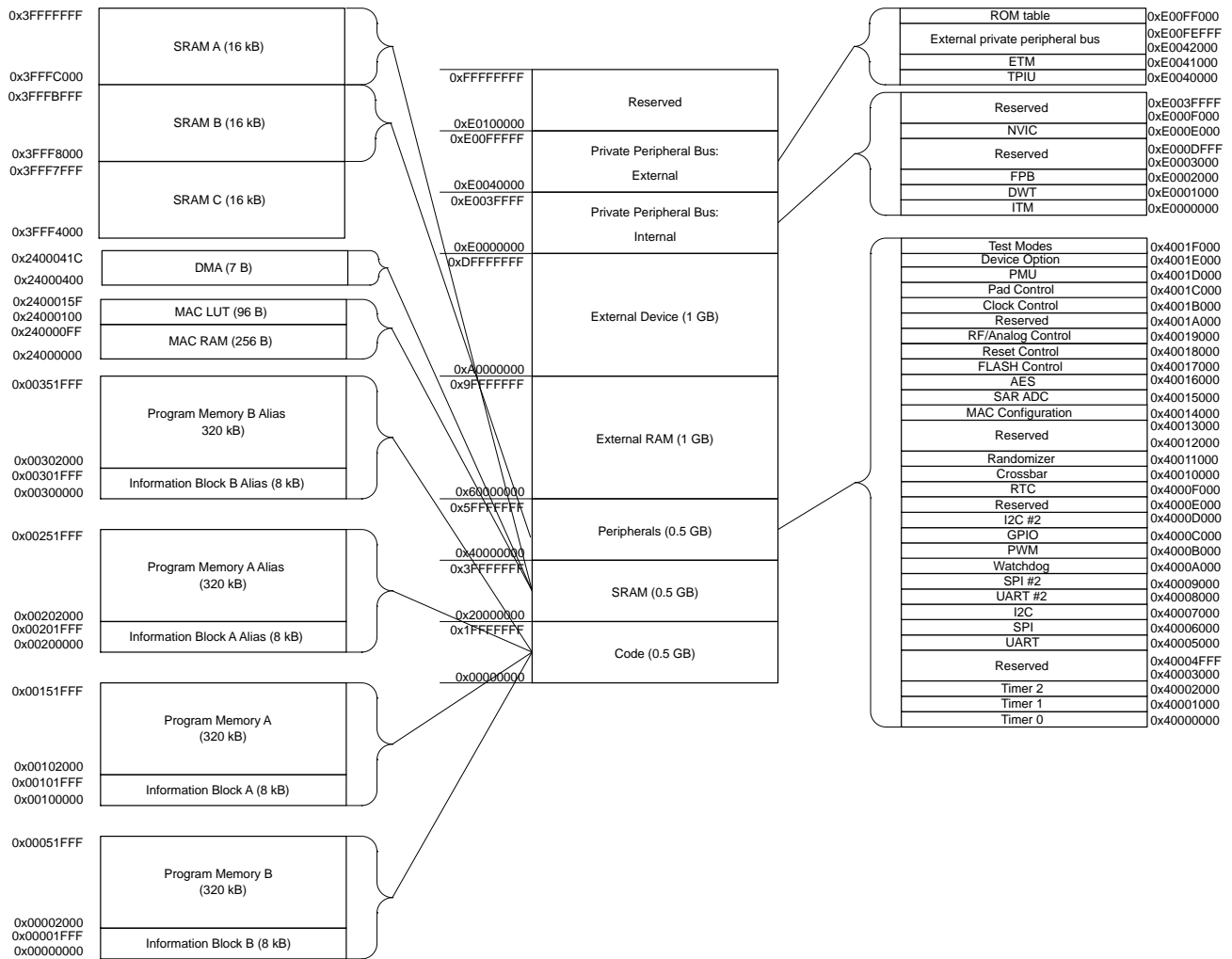
Figure 3. Memory Map
