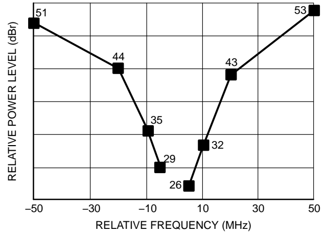
Figure 13. CW Mode Blocking / De-sensitization, 2.44 GHz
