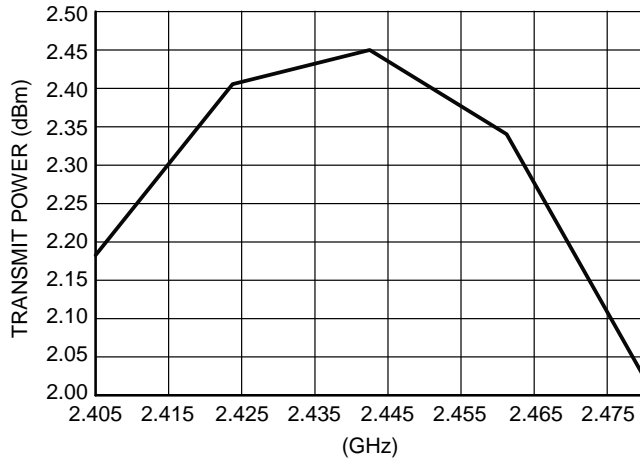
Figure 20. 1 V Mode Transmitter Output Power in CW Mode
