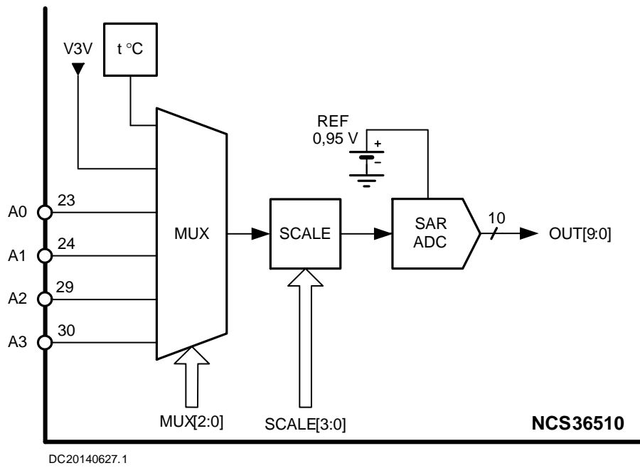
Figure 8. ADC Block Diagram
