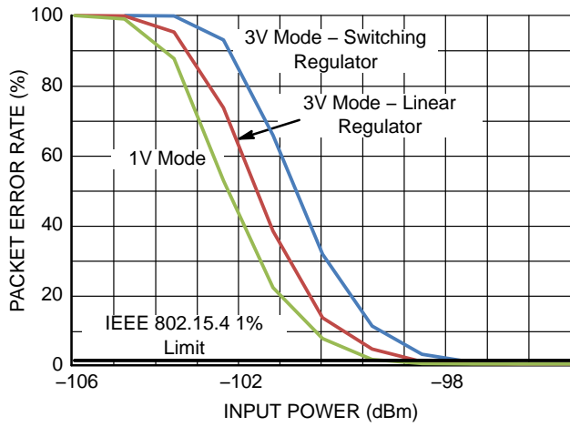
Figure 12. Packet Error Rate
