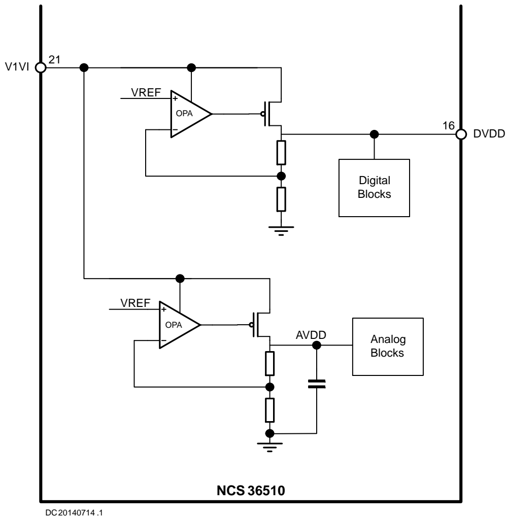
Figure 10. Linear Regulator System
