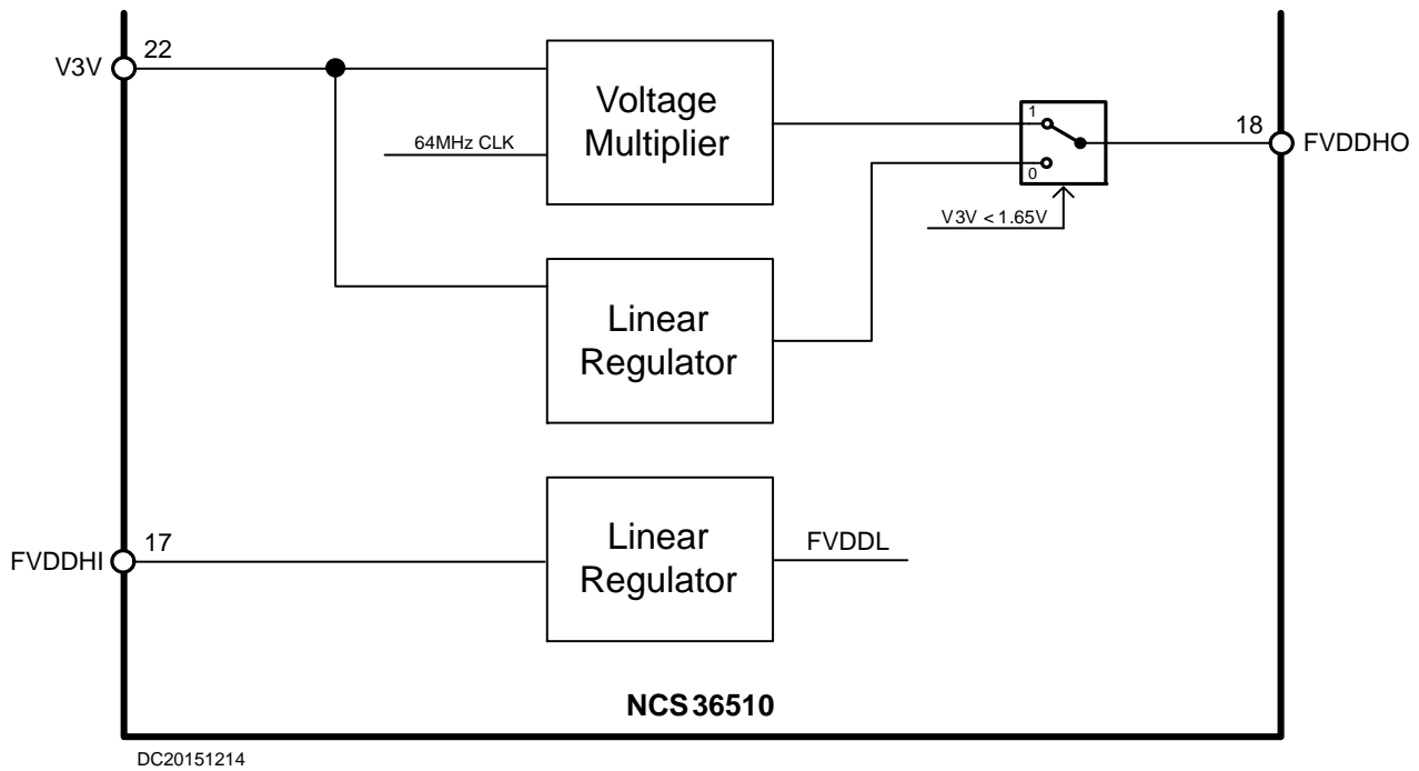
Figure 11. Flash Regulator System
