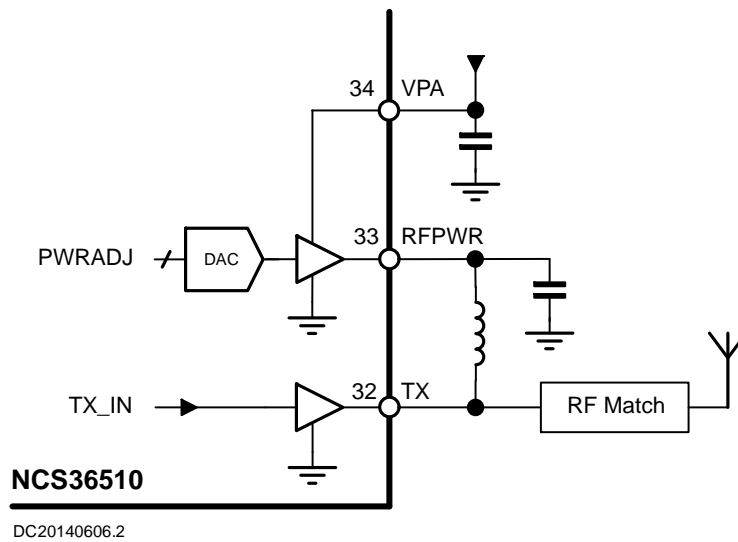
Figure 6. Transmitter
