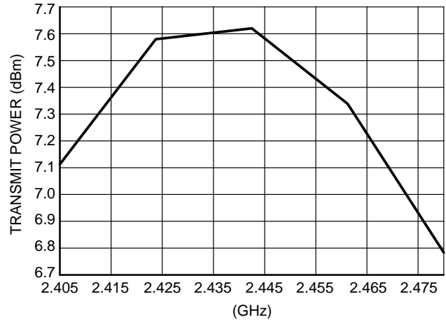
Figure 15. 3 V Mode with Linear Regulator Transmitter Output Power in CW Mode at Maximum Power
