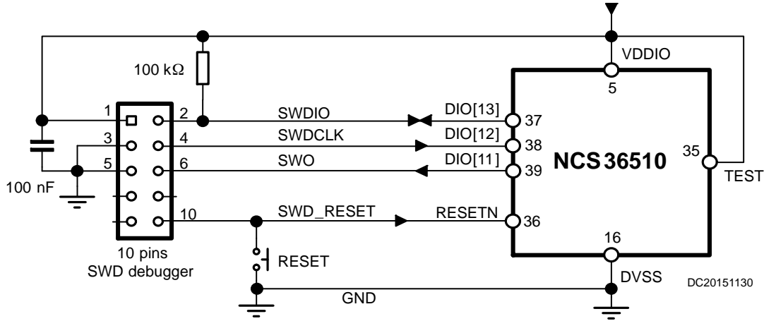
Figure 25. Debugger Connection Diagram
