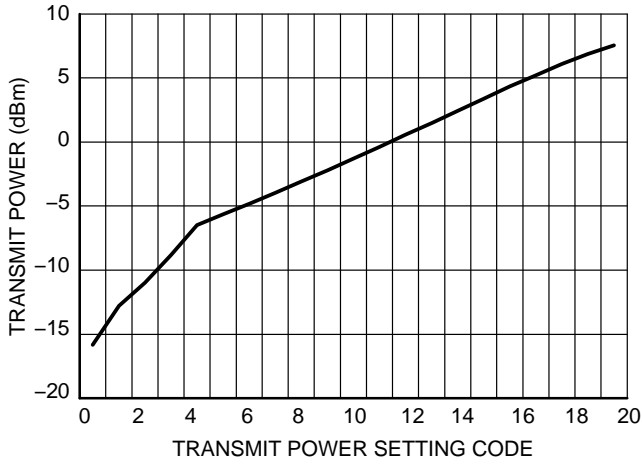
Figure 16. 3 V Mode with Switching Regulator Transmitter Power in CW Mode, 2.4425 GHz
