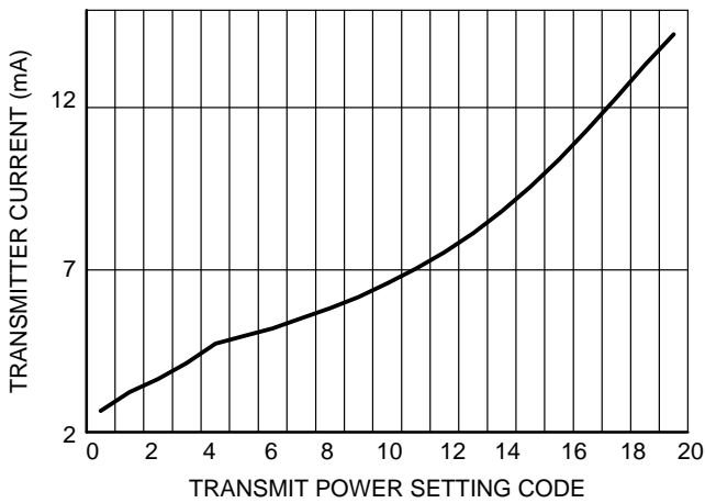
Figure 18. 3 V Mode with Switching Regulator Transmitter Current versus Power Setting, 2.4425 GHz
