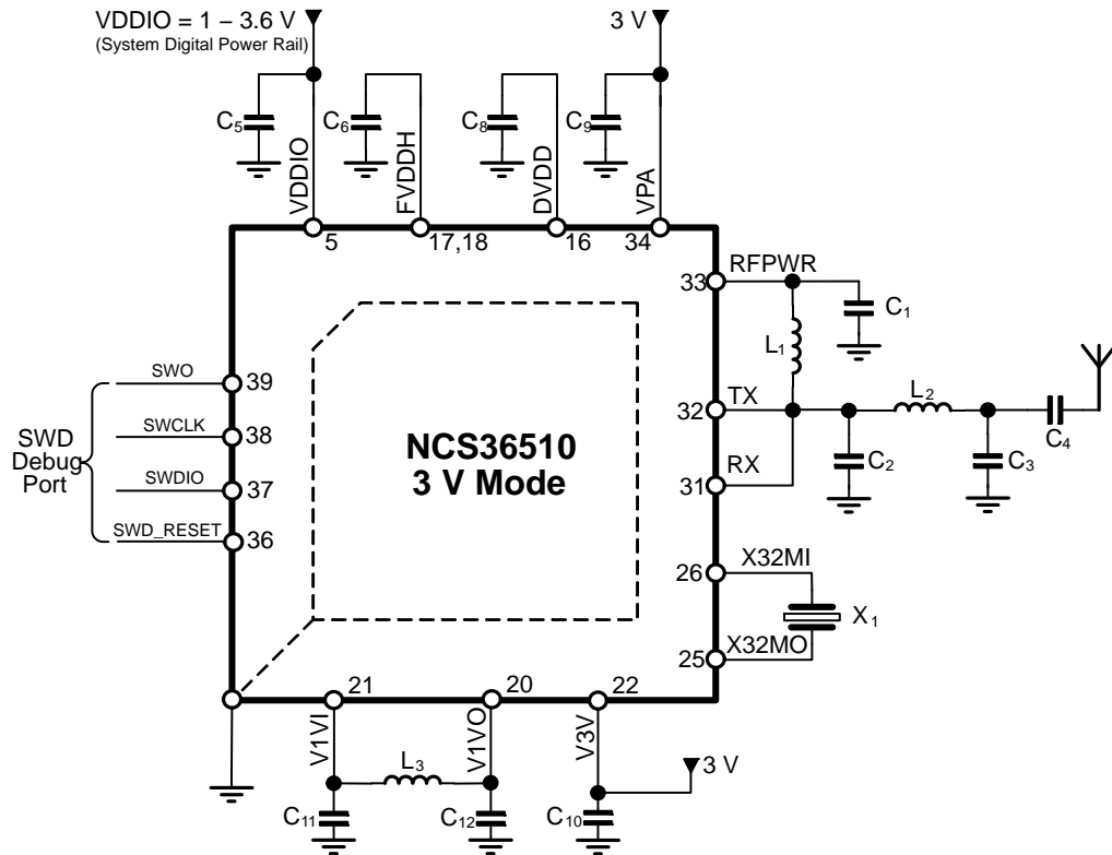
Figure 23. 3 V System Application Diagram
