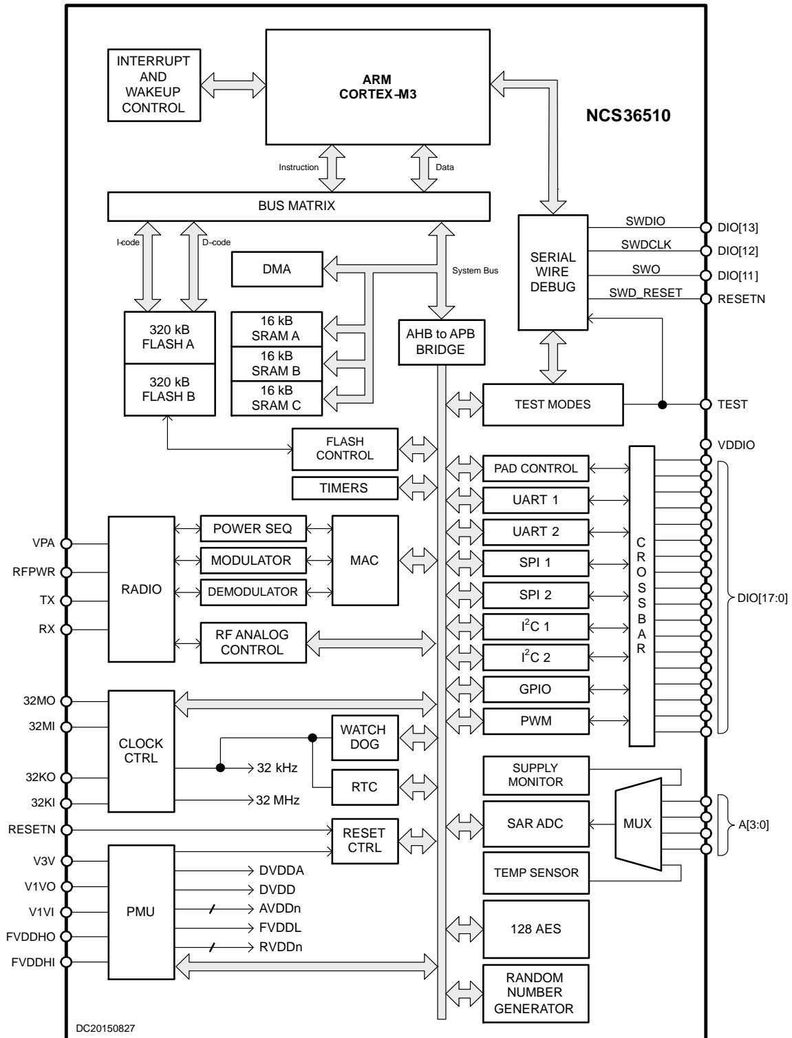
Figure 1. NCS36510 Block Diagram
