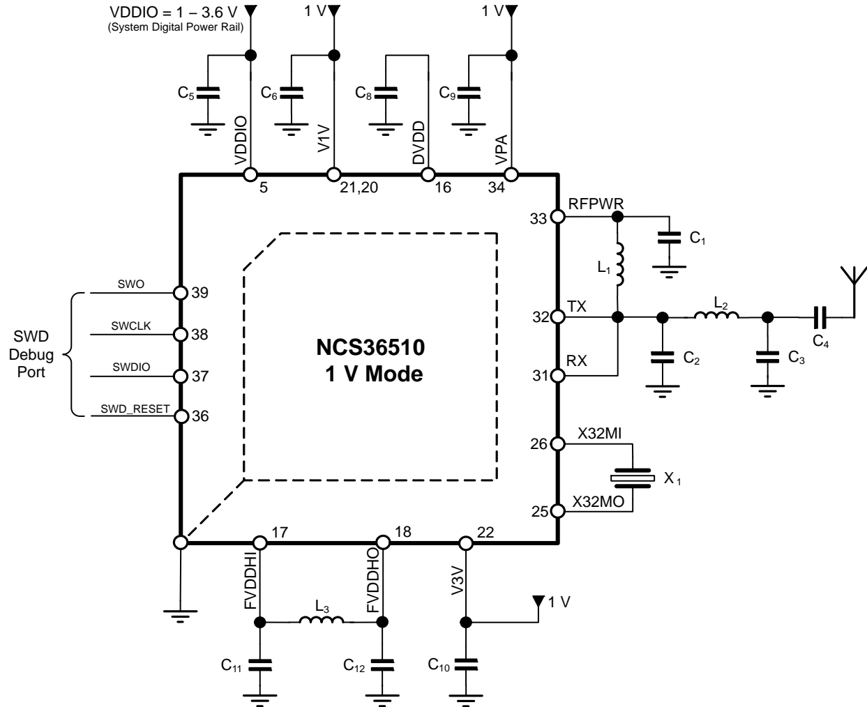
Figure 24. 1V System Application Diagram
