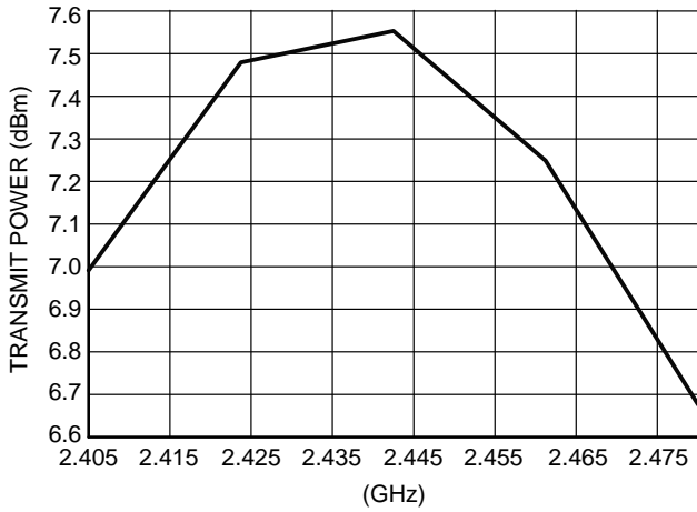
Figure 14. 3 V Mode with Switching Regulator Transmitter Output Power in CW Mode at Maximum Power
