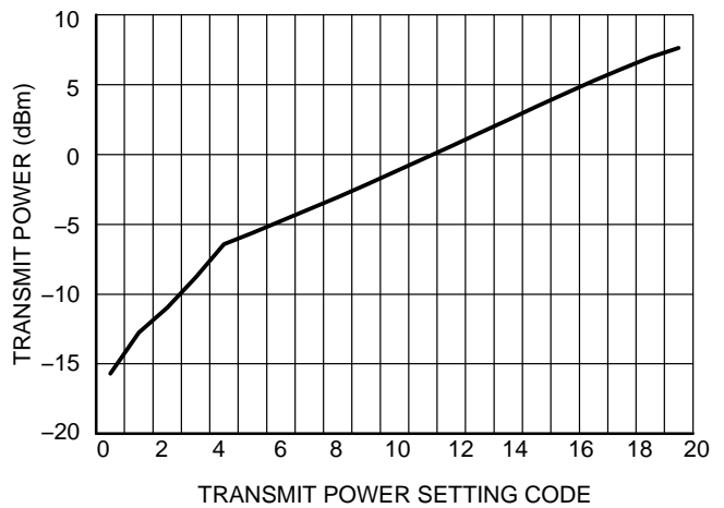
Figure 17. 3 V Mode with Linear Regulator Transmitter Power in CW Mode, 2.4425 GHz
