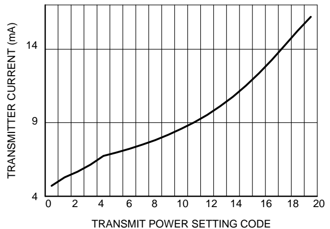
Figure 19. 3 V Mode with Linear Regulator Transmitter Current versus Power Setting, 2.4425 GHz
