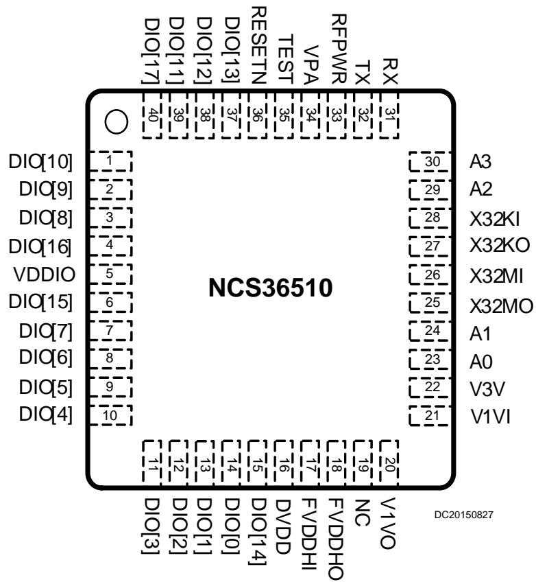
Figure 2. 40-Pin QFN Configuration (Top View)
