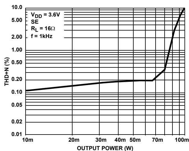
FIGURE 18. THD+N vs OUTPUT POWER
