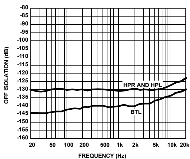
FIGURE 20. OFF ISOLATION vs FREQUENCY
