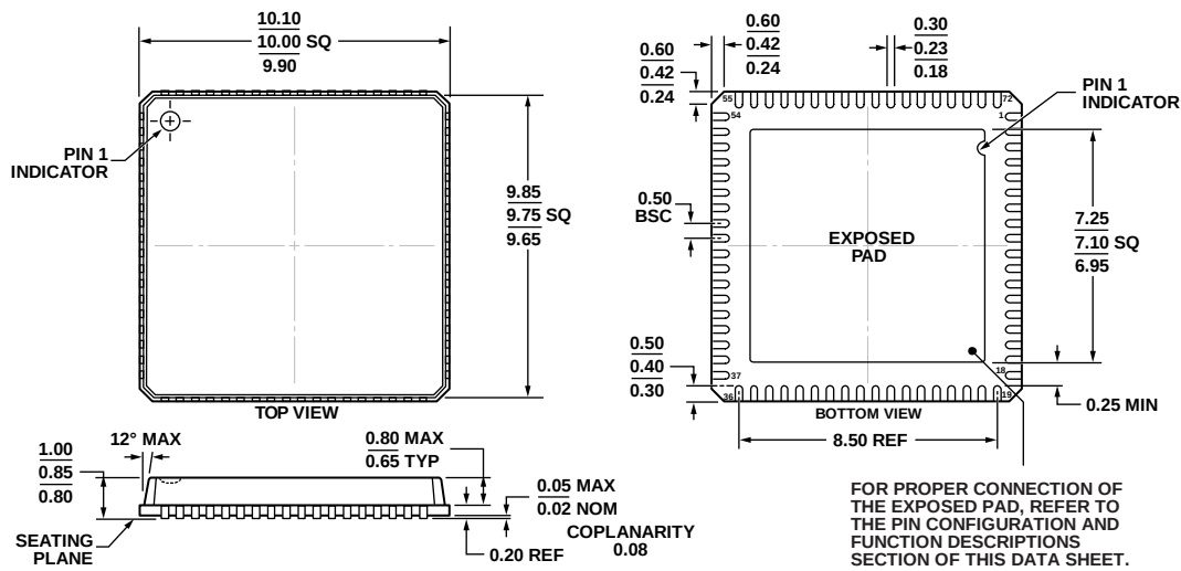
Figure 57. 72-Lead Lead Frame Chip Scale Package [LFCSP_VQ] 10 mm × 10 mm Body, Very Thin Quad (CP-72-4)
