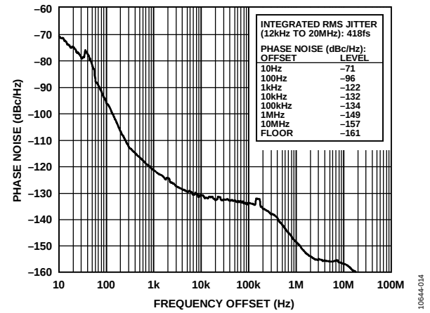
Figure 14. Absolute Phase Noise (Output Driver = 1.8V CMOS), f_R = 2 kHz, f_{OUT} = 70.656 MHz, DPLL Loop BW = 10 Hz, f_{SYS} = 19.2 MHz TCXO
