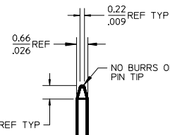
DETAIL X SCALE 5:1 SEE NOTE 10
