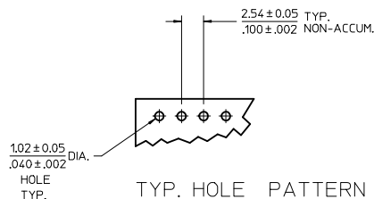
TYP. HOLE PATTERN FOR 1.57/.062 THK. PCB
