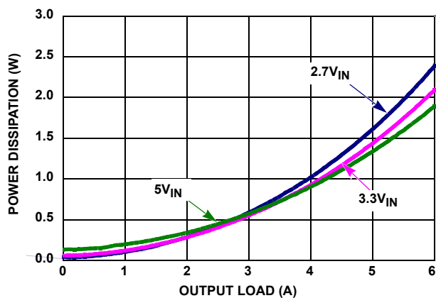
FIGURE 44. POWER DISSIPATION vs LOAD, 1.8V , T_A = +25^\circ C
