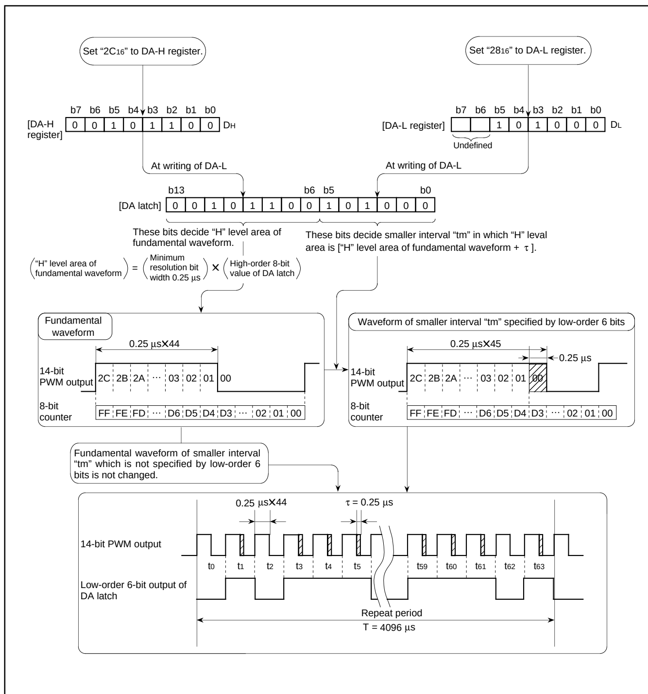
Fig. 24. 14-bit PWM Output Example ( f(X_{IN}) = 8 MHz)
