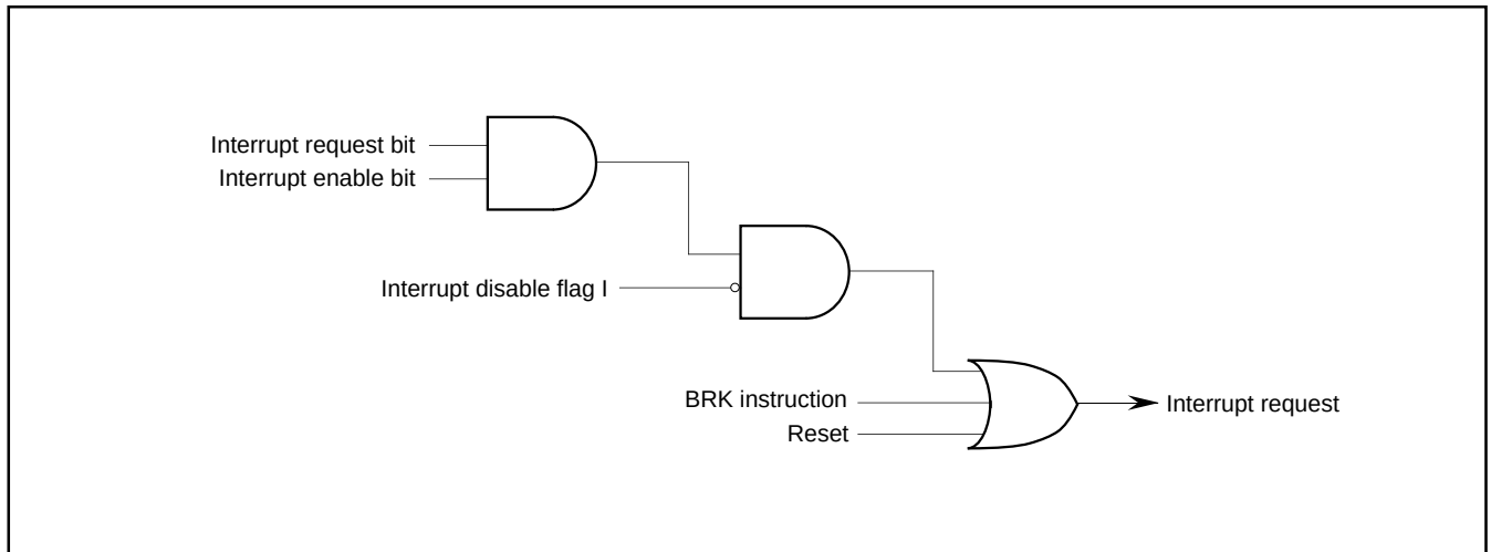
Fig. 9. Interrupt Control
