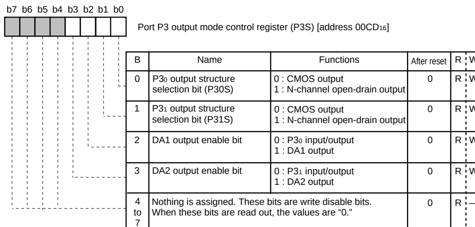
Fig. 32. Port P3 Output Mode Control Register
