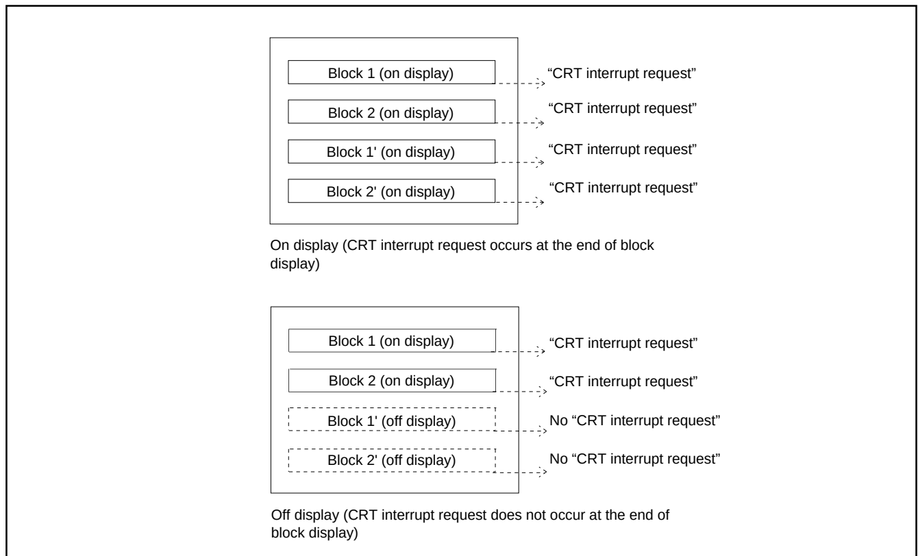
Fig. 47. Timing of CRT Interrupt Request
