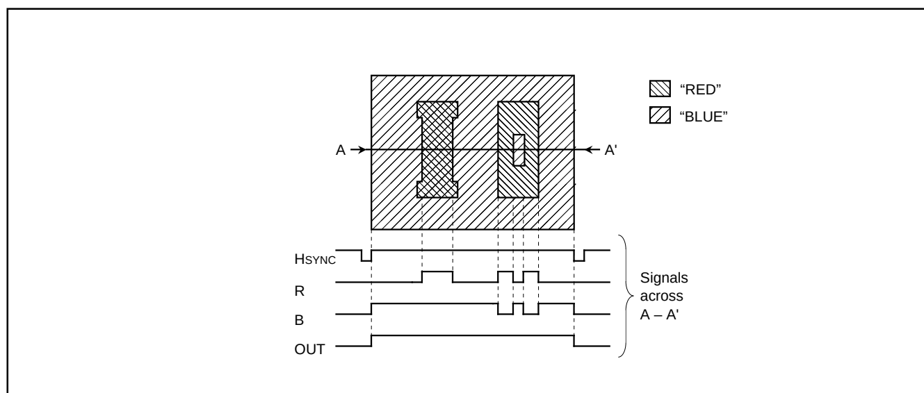
Fig. 49. Example of Raster Coloring
