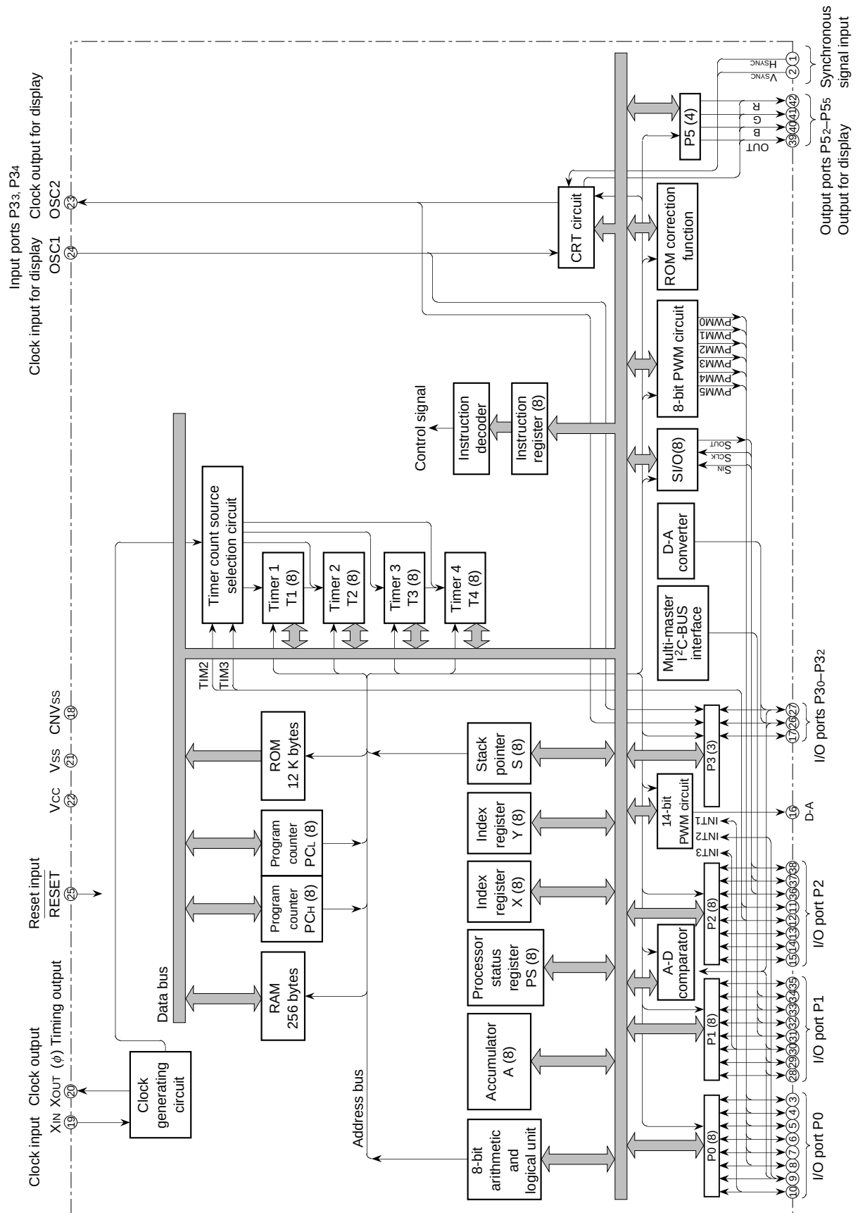
FUNCTIONAL BLOCK DIAGRAM of M37224M3-XXXSP
