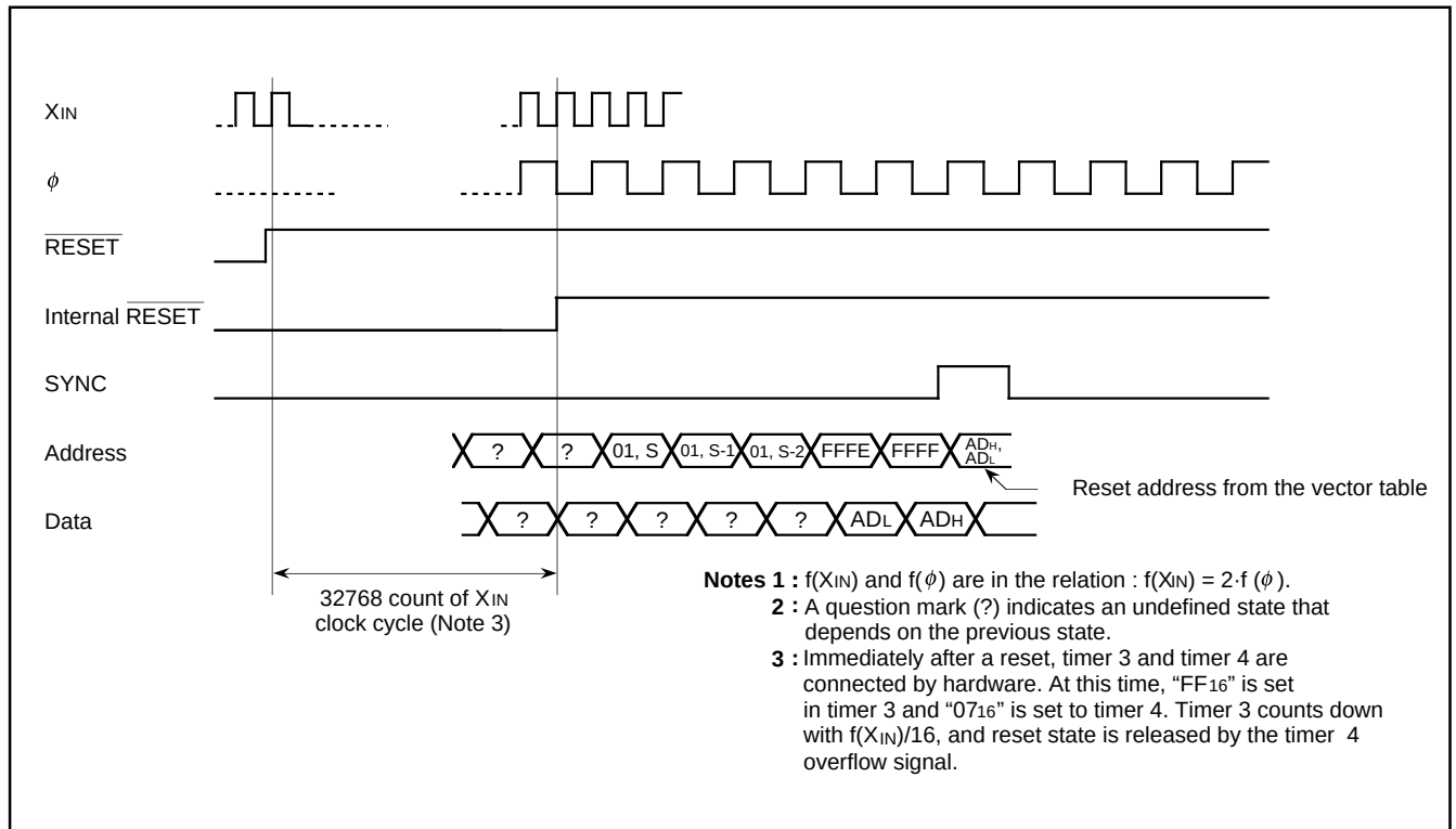
Fig. 53. Reset Sequence
