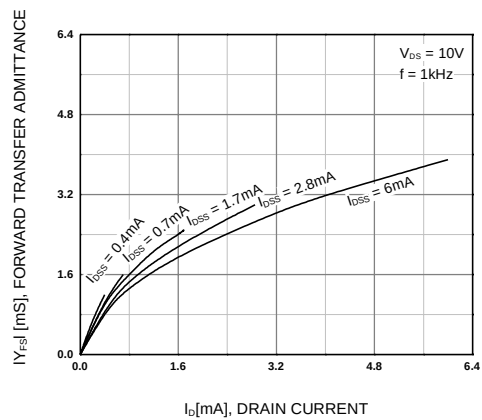
Figure 5. |Y_{fs}| - I_D
