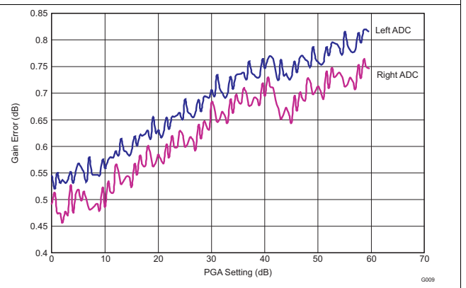
Figure 8. ADC Gain Error vs PGA Gain Setting
