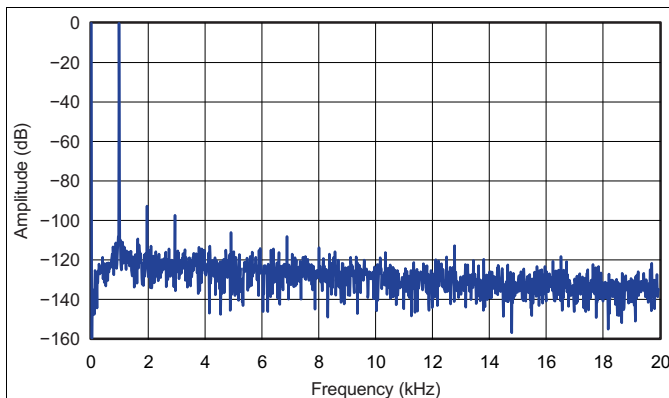
Figure 33. DAC to Line Output FFT at 1-kHz Signal Plot
