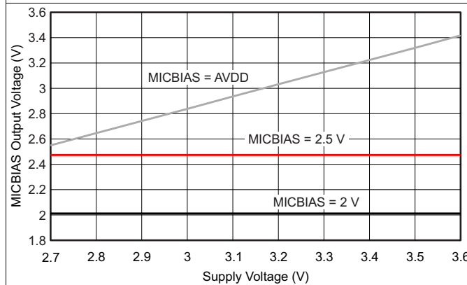
Figure 9. MICBIAS Output Voltage vs AVDD
