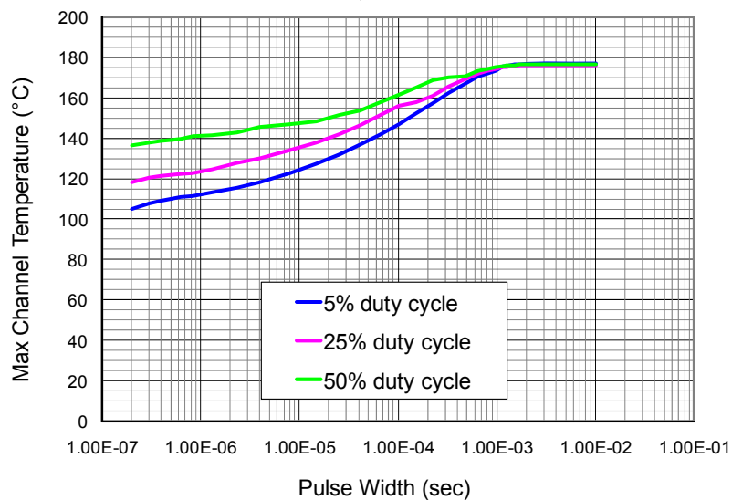
Max Channel Temperature Tbase = 85 °C, Pdiss = 3 w/mm
