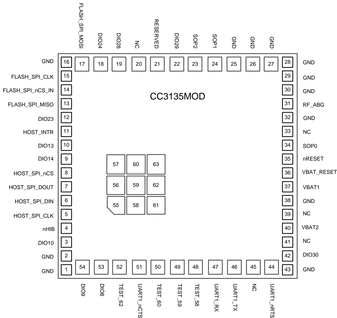
Figure 4-1. CC3135MOD Pin Diagram Bottom View
