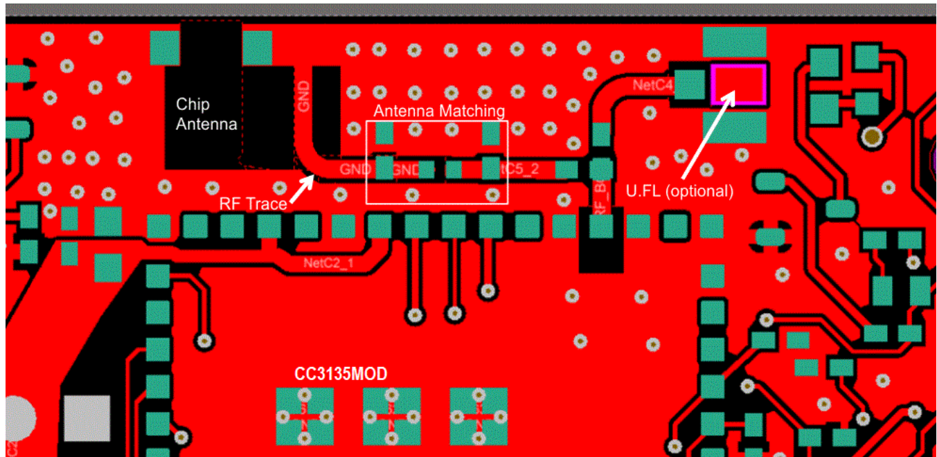
Figure 7-4. RF Section Layout
