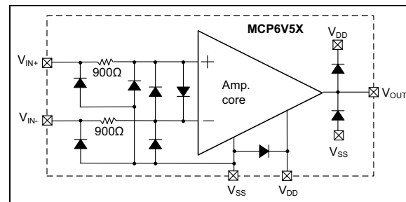
FIGURE 4-5: Simplified Analog Input ESD Structures.
