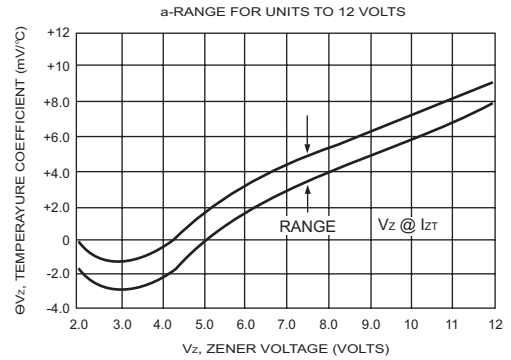
FIG.7- TEMPERATURE COEFFICIENTS
