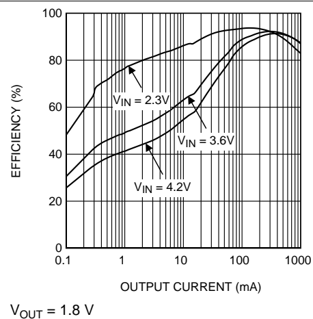
Figure 12. Efficiency vs Output Current, ECO Mode
