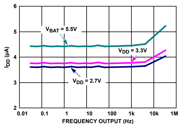
FIGURE 9. F_{OUT} vs I_{DD}
