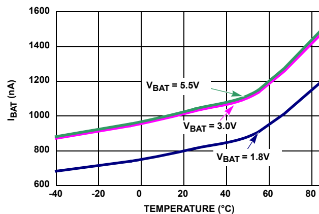
FIGURE 5. I_{BAT} vs TEMPERATURE ( V_{DD} = 0V )
