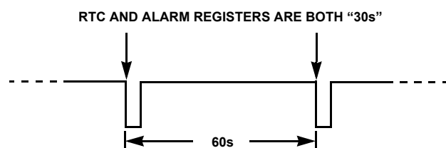
FIGURE 16. \overline{\text{IRQ}}/\text{F}_{\text{OUT}} WAVEFORM
