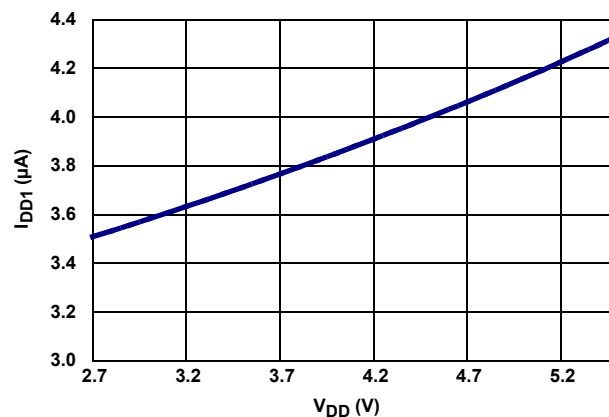
FIGURE 7. I_{DD1} vs V_{DD}
