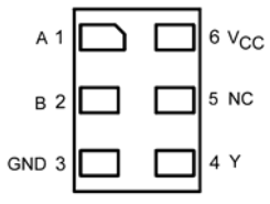
Figure 3. MicroPak™ (Top Through View)
