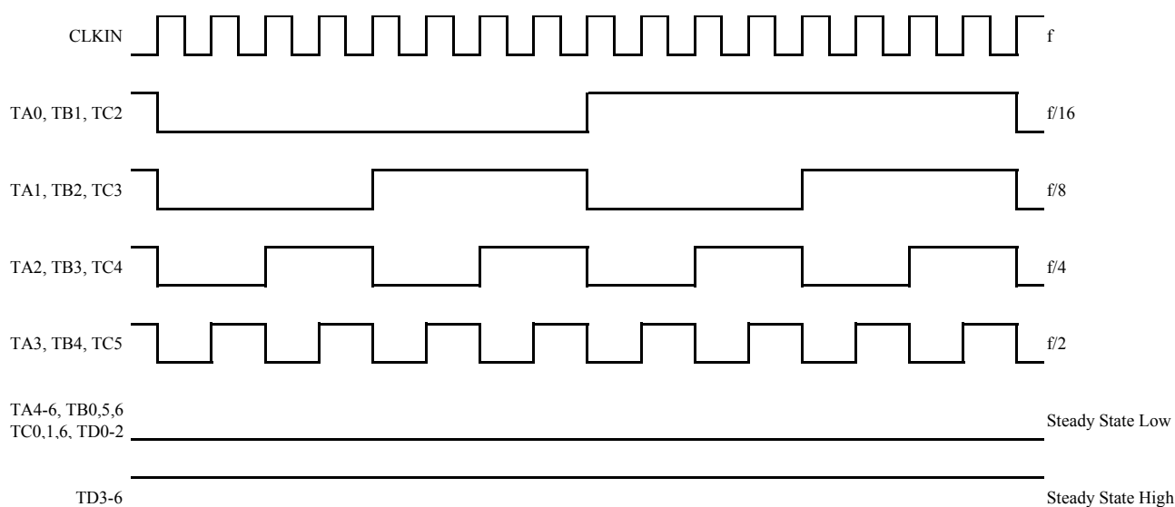
Fig.1 16 Grayscale Pattern
