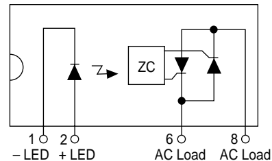
CPC1965Y Pinout
