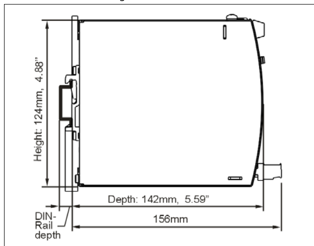
Fig. 23-2 Side view
