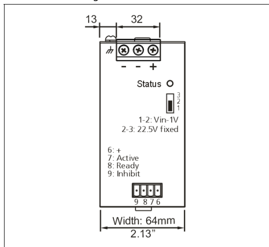
Fig. 23-1 Front view
