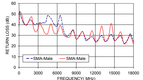
086-3SM+ RETURN LOSS
