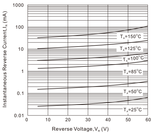
Fig. 3 - Reverse Characteristics
