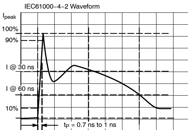
Figure 12. IEC61000-4-2 Spec
