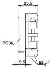
Dimensioned drawing
