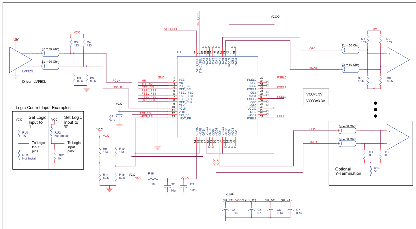
FIGURE 6. 873991-147 SCHMATIC LAYOUT
