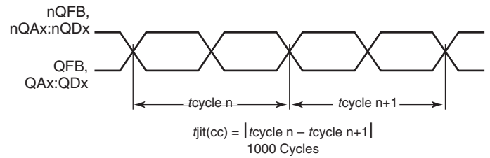
CYCLE-TO-CYCLE JITTER
