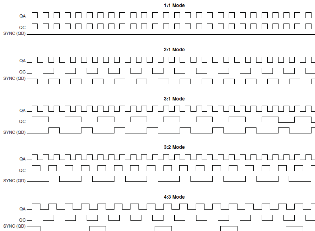
FIGURE 1. TIMING DIAGRAMS
