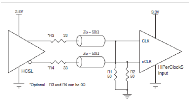
FIGURE 4E. HiPerClockS CLK/nCLK INPUT DRIVEN BY A 3.3V HCSL DRIVER
