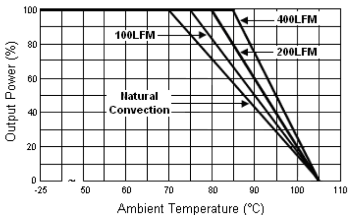
Derating Curve
