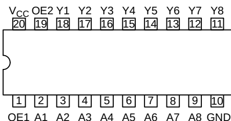
20-Lead (Top View)
