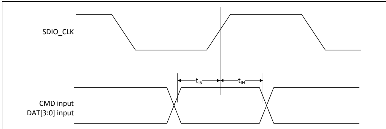
Figure 46: SDIO Bus Input Timing (SDR Modes)
