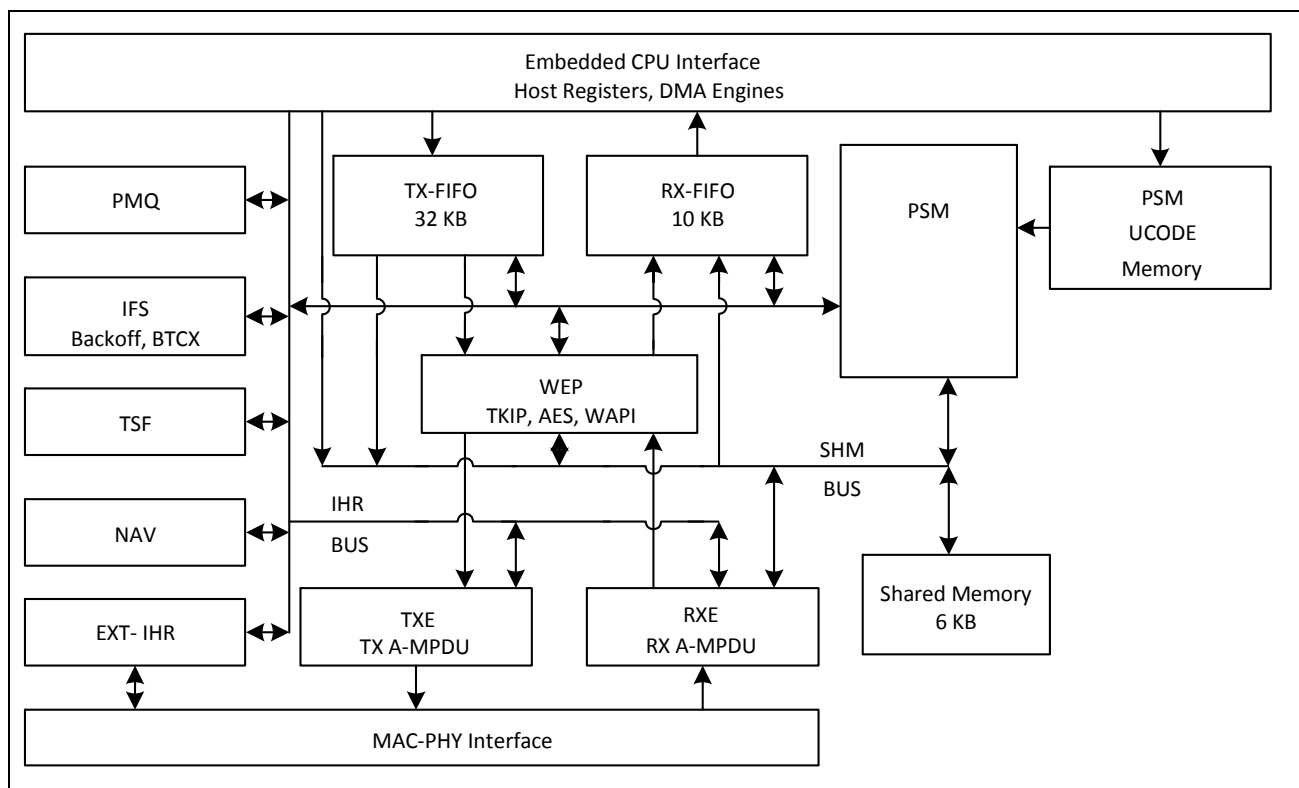
Figure 35: WLAN MAC Architecture
