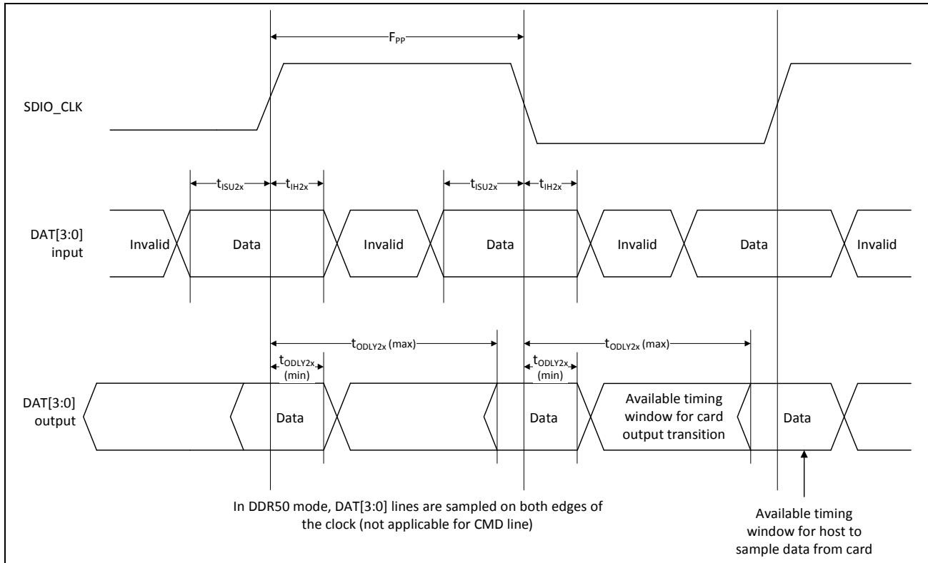
Figure 51: SDIO Data Timing (DDR50 Mode)
