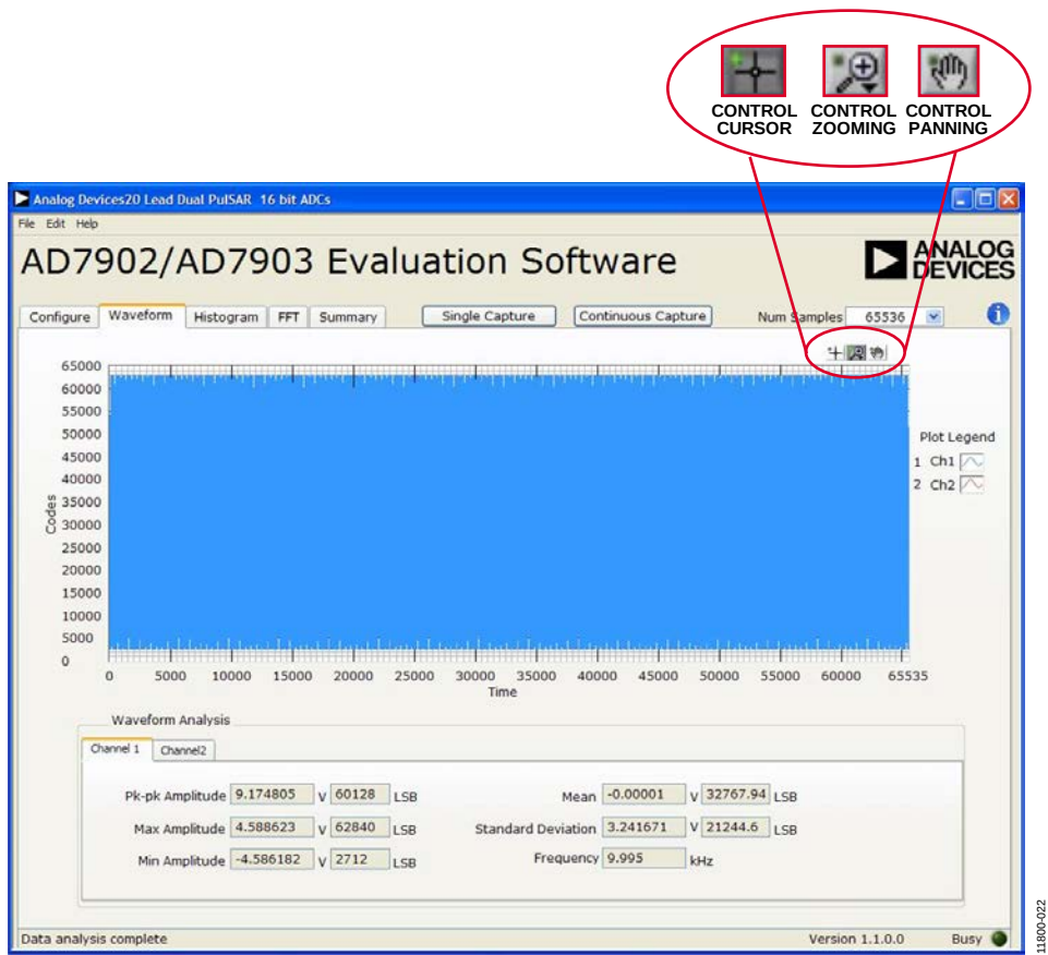
Figure 22. Waveform Tab
