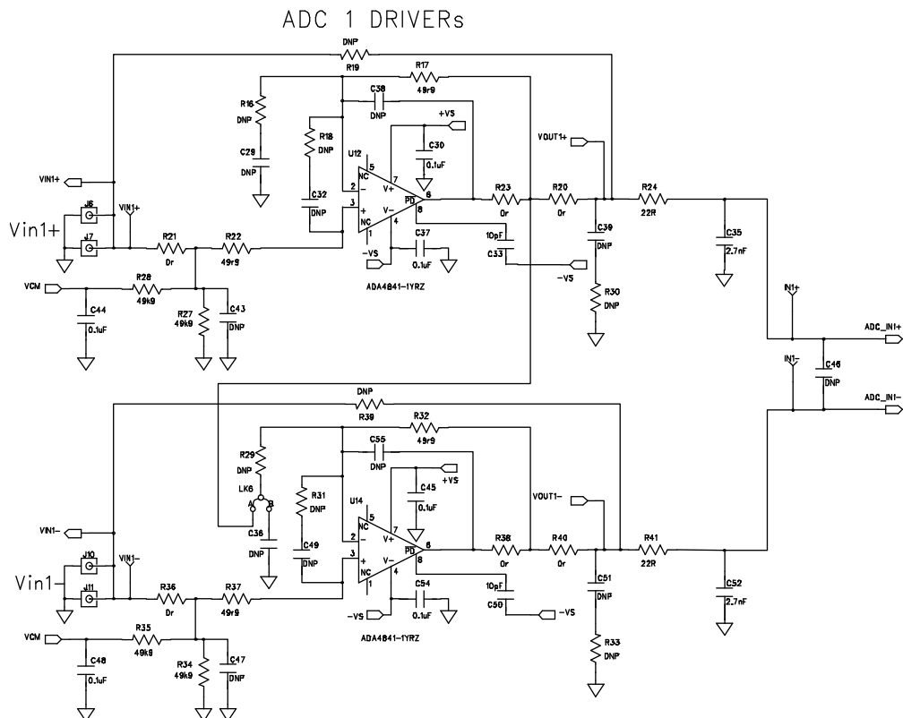
Figure 26. Schematic, Page 1
